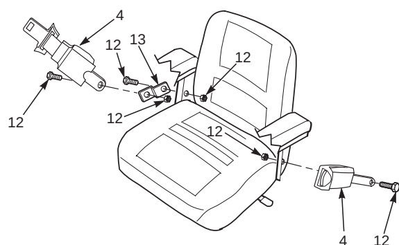
Seat Assy. With Black Arm Rest
