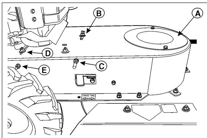
Figure 19 - Belt Adjustments
