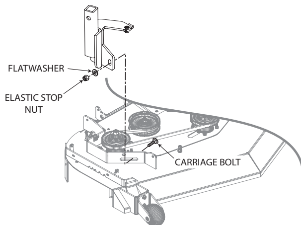
Figure 2-3. Blower Mounting Post Installation
