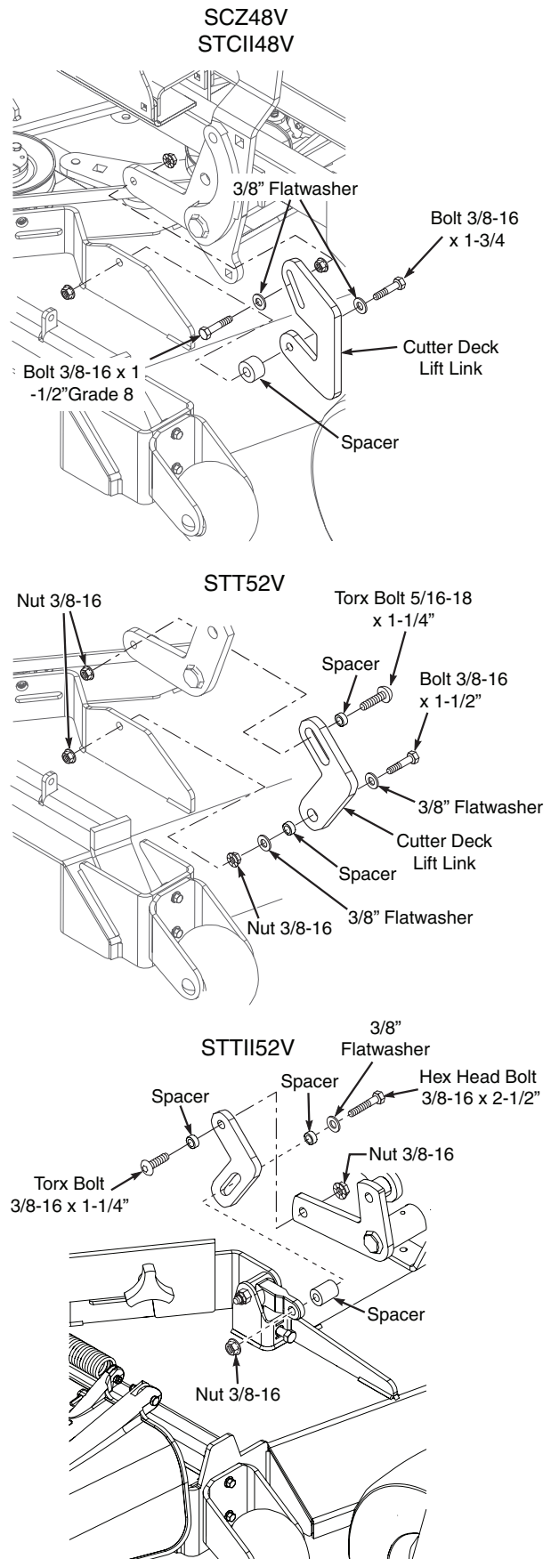
Figure 2-4. Cutter Deck Lift Link Installation
