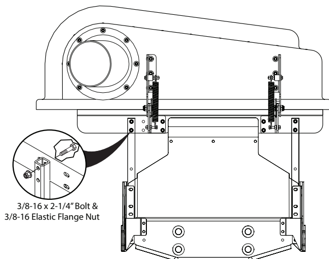
Figure 2-8. Hitch Assembly Installation
