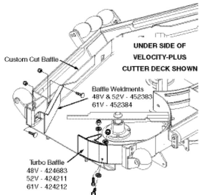
Figure 2-2. Grass Catcher Baffles
