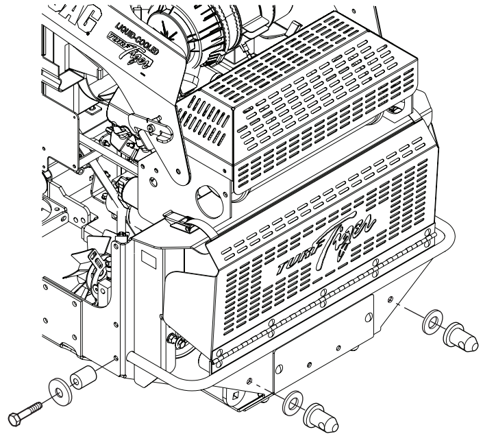
Figure 2-12. STT / STTII Hopper Mounting Hardware Install
