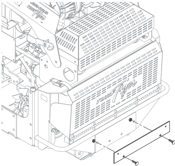
Figure 2-10. STT Hopper Mounting Hole Template
