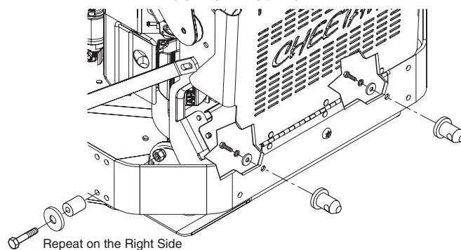
Figure 2-9. Hopper Mounting Hardware Install
