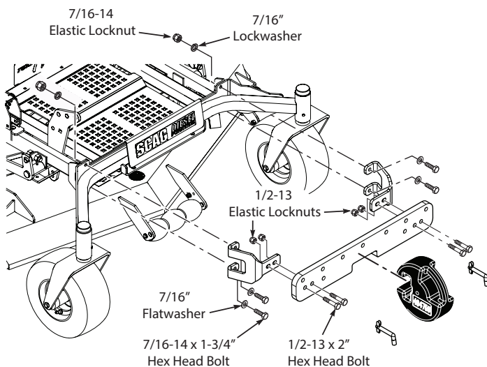
Figure 2-17. STT-Diesel, STTII & SCZ61" Weight Bar Install
