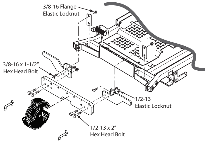
Figure 2-16. STT Front Weight Bar Installation
