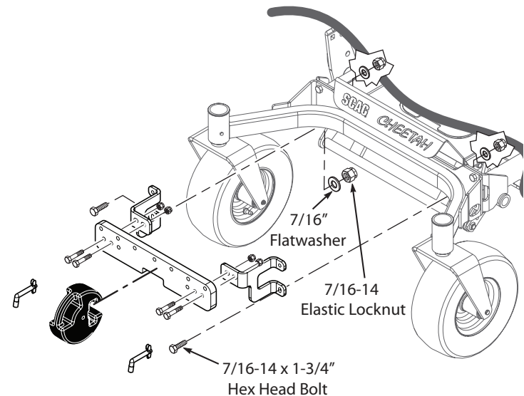
Figure 2-15. SCZ48/52" & STCII Front Weight Bar Install
