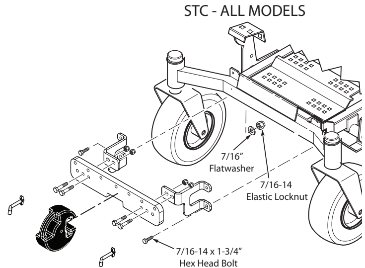
Figure 2-14. STC Front Weight Bar Installation
