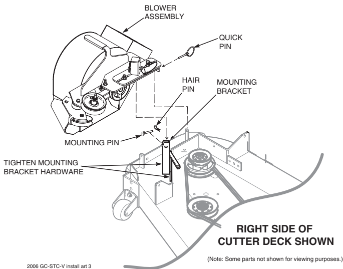
Figure 2-5. Blower Installation
