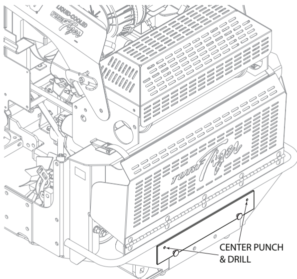
Figure 2-11. STT Hopper Mounting Holes
