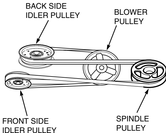
Figure 2-6. Belt Routing
