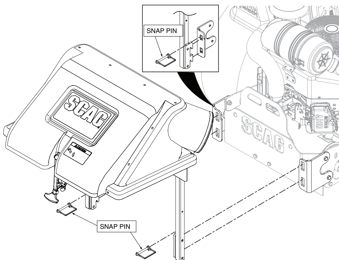
Figure 2-17. SFZ / SFZP / SPZ Hood Assembly Installation
