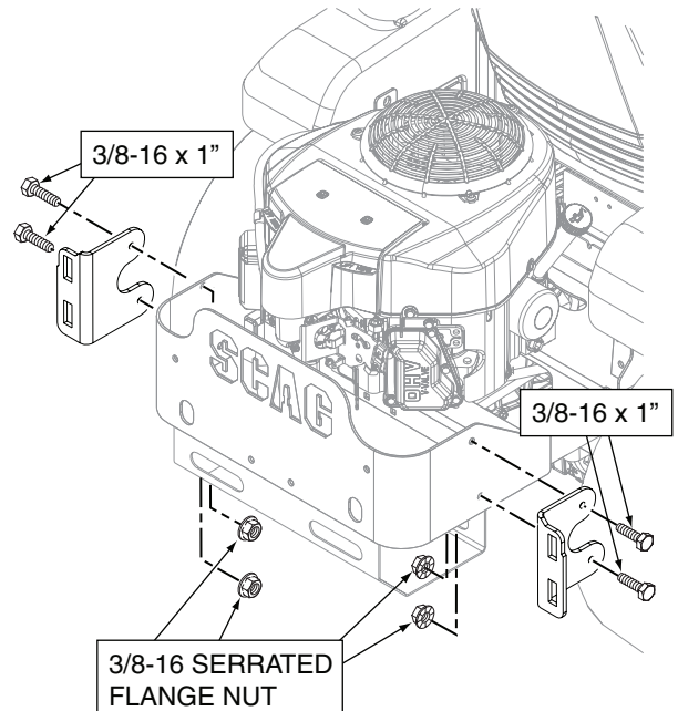
Figure 2-13. SZL36 GC Mounting Bracket Installation
