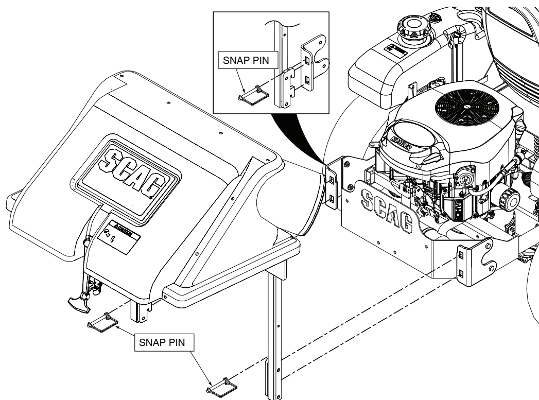
Figure 2-18. SZL / SFZ / SPZ Hopper Mounting Holes
