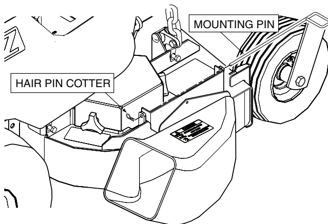
Figure 2-12. GC Discharge Boot Installation
