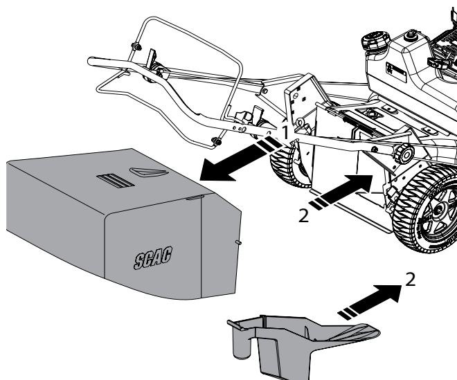
Figure 6-7. Mulch Conversion
