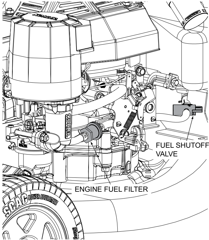
Figure 7-3. Fuel Filter
