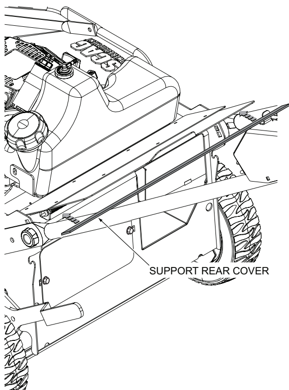
Figure 6-1. Lift and Support Rear Cover
