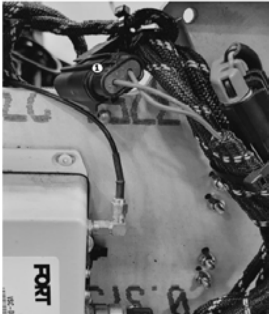
Figure 6-8. Fort Receiver Fuse
