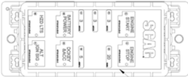
Figure 6-6. Fuse and Relay Box
