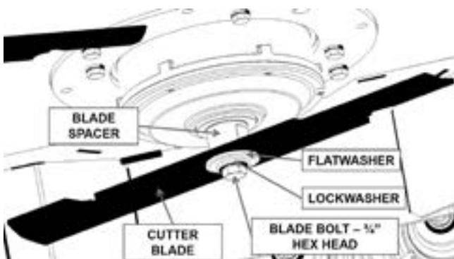
Figure 6-2. Blade Replacement
