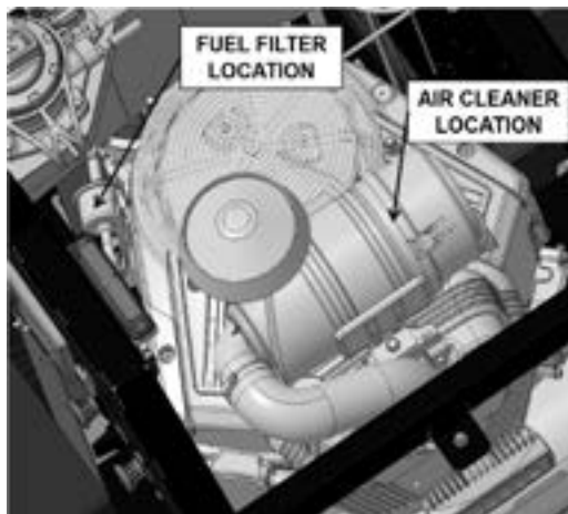
Figure 6-4. Fuel Filter and Air Cleaner Location
