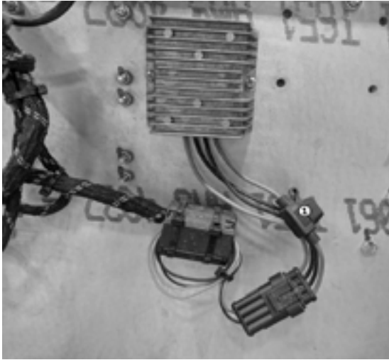
Figure 6-10. DCDC Converter Fuse
