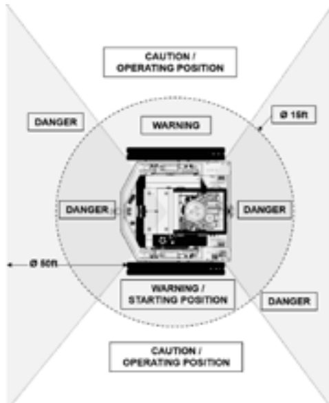
Figure 4-16. Operator Area
