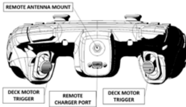
Figure 4-4. Fort Remote Controls Cont.
