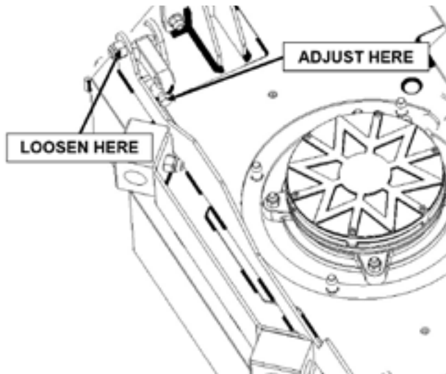
Figure 5-3. Cutter Deck Pitch Adjustment
