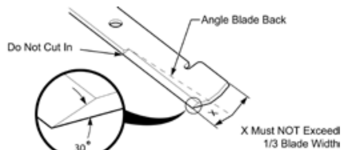
Figure 6-1. Blade Sharpening
