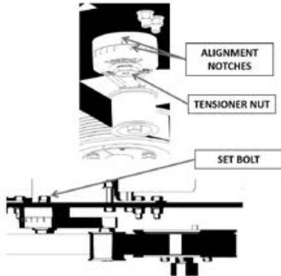
Figure 5-4. Alternator Belt Tensioner Adjustment
