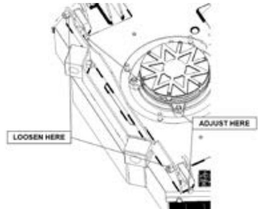
Figure 5-2. Cutter Deck Level Adjustment
