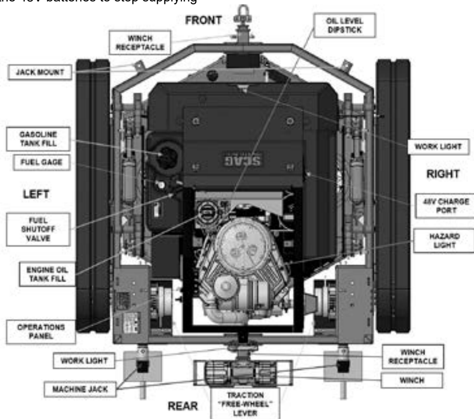
Figure 4-1. Machine Overview
