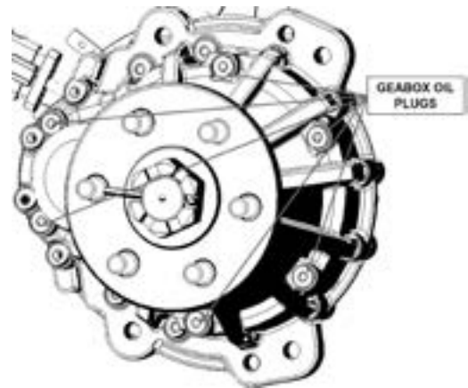
Figure 6-5. Gearbox Oil Plug Locations
