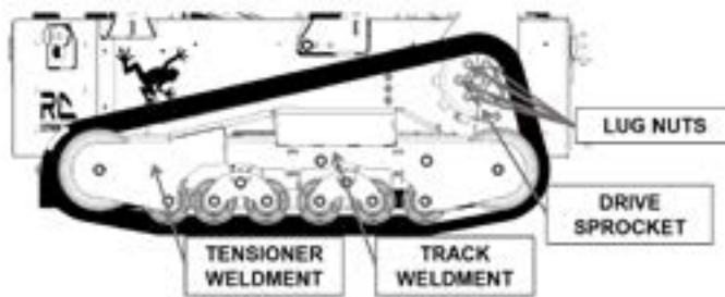
Figure 6-3. Track Assembly
