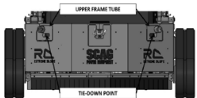
Figure 2-2. Machine Tie-Down Points
