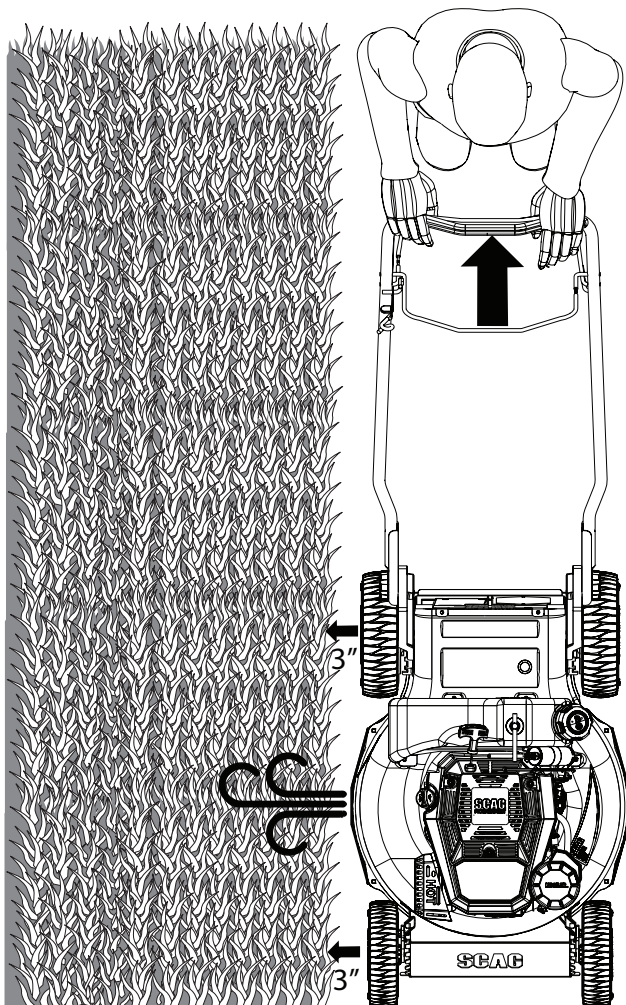
Figure 2-1. Blade Stop
