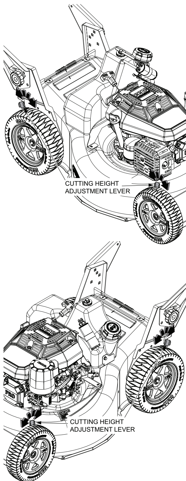
Figure 4-5. Adjusting Cutting Height
