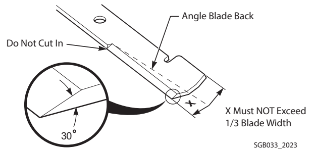
Figure 7-5. Blade Sharpening
