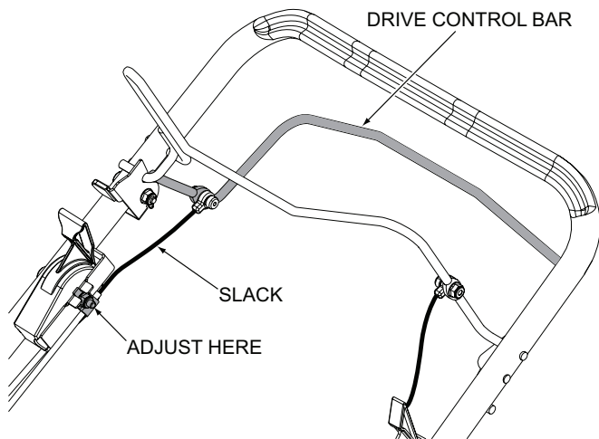
Figure 6-6. Deck Drive Cable Adjustment
