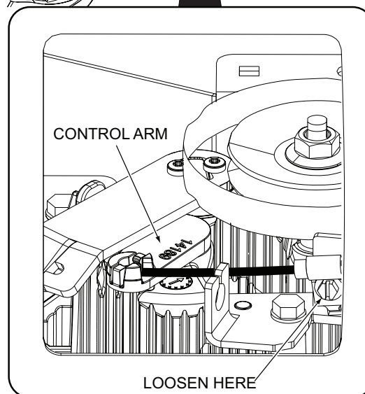
Figure 6-2. Transmission Access
