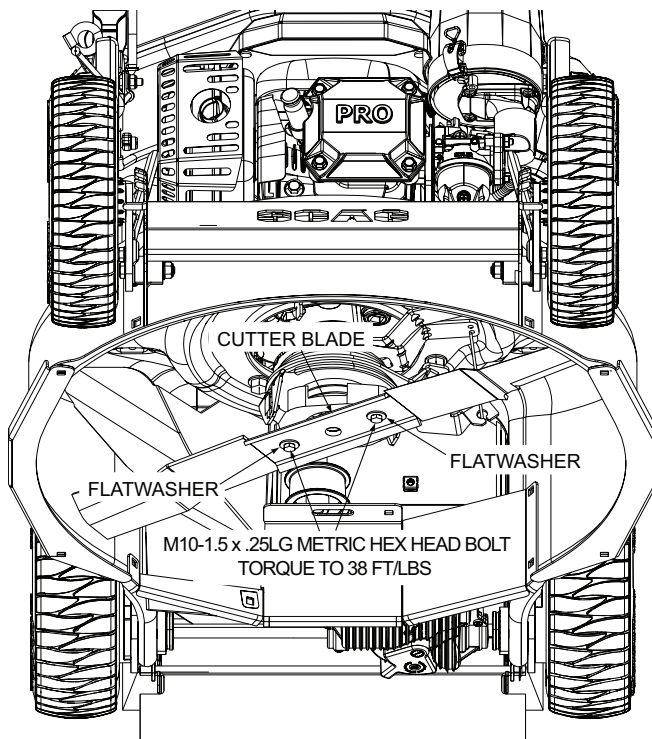
Figure 7-6. Blade Replacement
