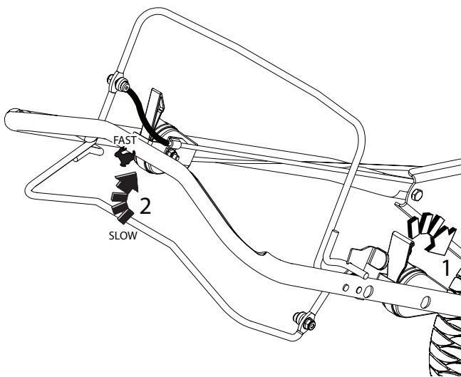
Figure 4-3. Travel Controls
