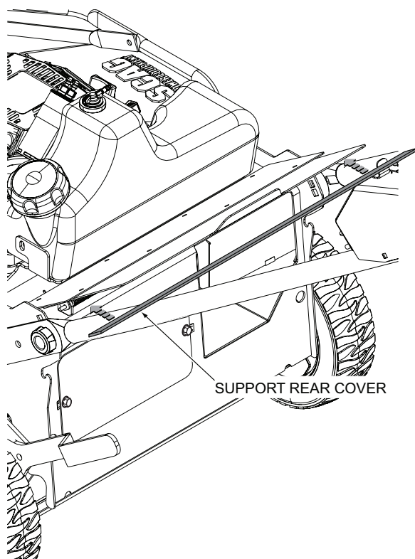
Figure 6-1. Lift and Support Rear Cover
