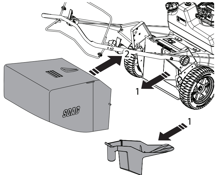
Figure 6-8. Bagging Grass.
