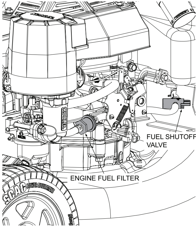
Figure 7-3. Fuel Filter
