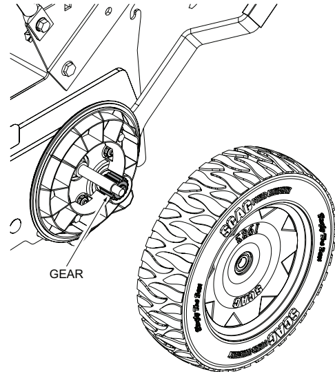
Figure 7-7. Rear Wheels
