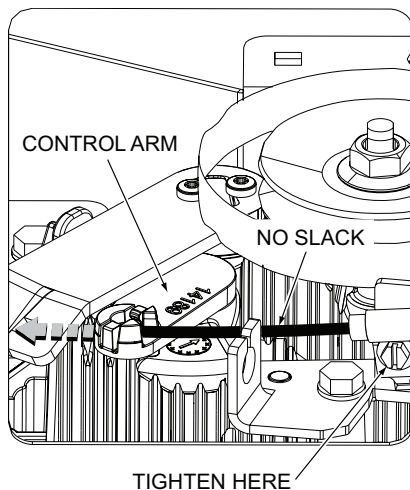
Figure 6-4. Transmission Control Arm and Spring
