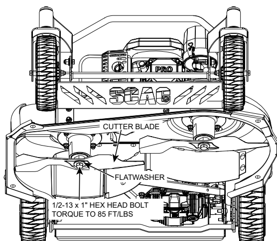
Figure 7-7. Blade Replacement
