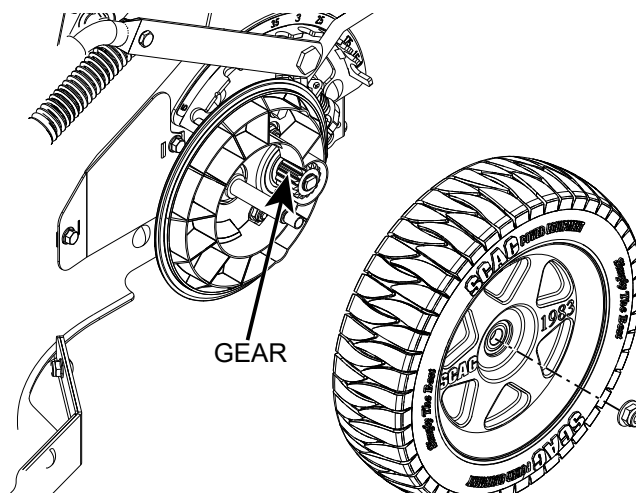
Figure 7-8. Rear Wheels
