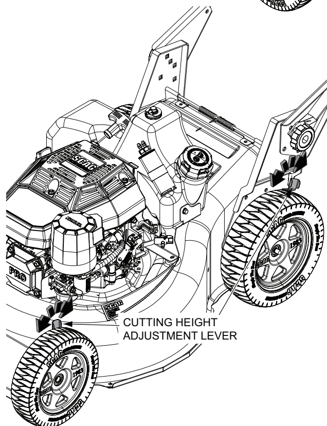
Figure 4-5. Adjusting Cutting Height
